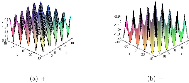
Fig. 3: The 3D graphs of (3.18) as a = 2.5 , b = -2 , c = 4 , C = -0.3 , x \in (-14, 14) .
